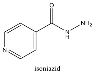
Scheme-1: INH ligand.
