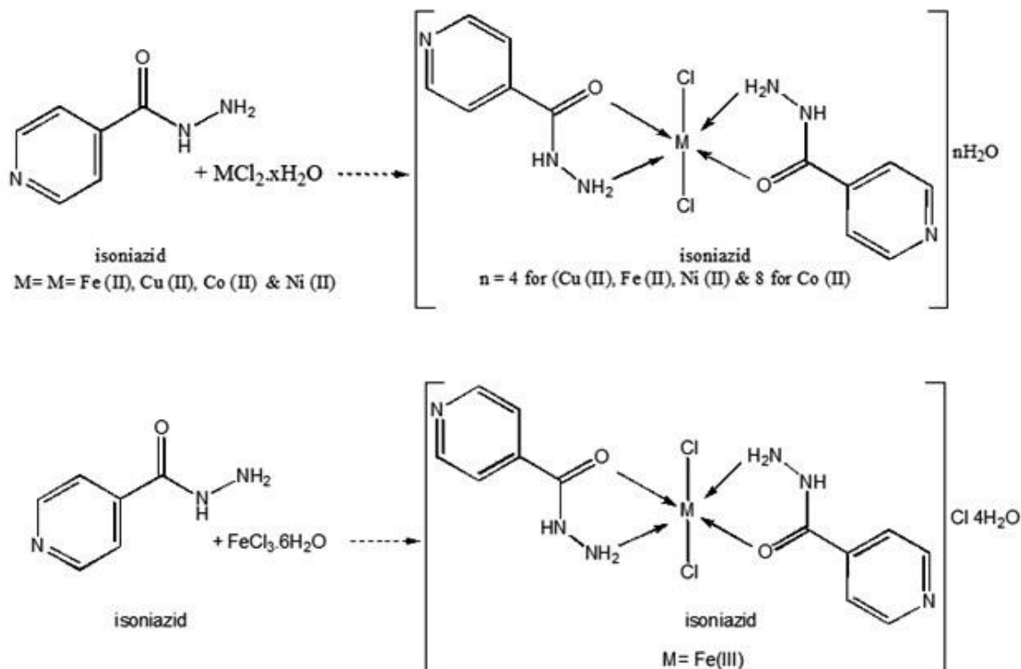
Scheme-2: Predicted structures for complexes.
